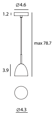
Castle Pendant XS SG-623CP G9 1 x Max 35W Halogen bulb Materials : concrete, steel
