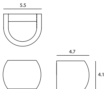
Castle Wall R LED OUTDOOR SLD-7034CWO LED 1 x 5W (3000K, CRI90, 440lm) built-in driver Materials : concrete, steel
