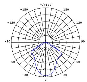
CASTLE P M UNIT: °cd AVERAGE BEAM ANGLE (50%) : 115.3 DEG
