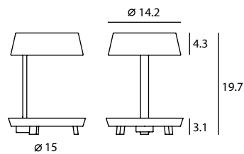
Carry Table SQ-6350MDU E26 2 x Max 60W on/off push switch Materials : steel, beech Color : matte black & red / matte white & beech USB charger
