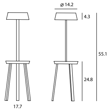
Carry Floor SQ-6350MFU E26 2 x Max 60W on/off push switch Materials : steel, beech Color : matte black & red / matte white & beech USB charger
