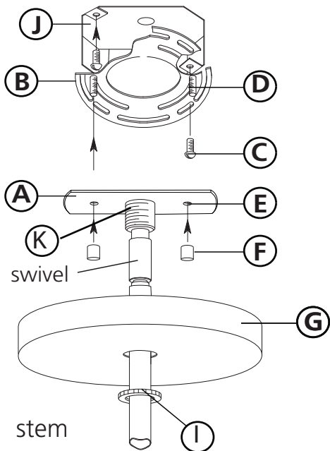
DRAWING 2-MOUNTING
