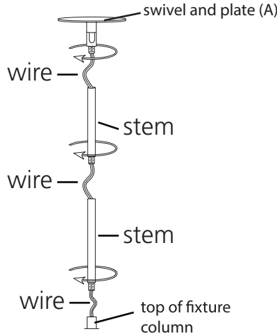
DRAWING 2-MOUNTING
