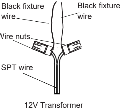
DRAWING 2- Multiple fixture wiring
