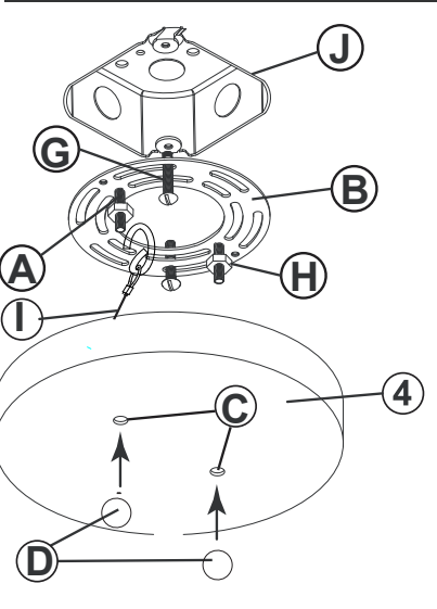
Drawing 3– Mounting Detail
