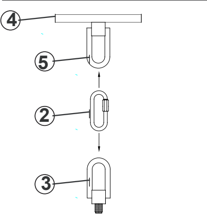
Drawing 3– Mounting Detail
