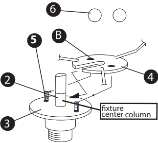
Drawing 5 - Shade mounting
