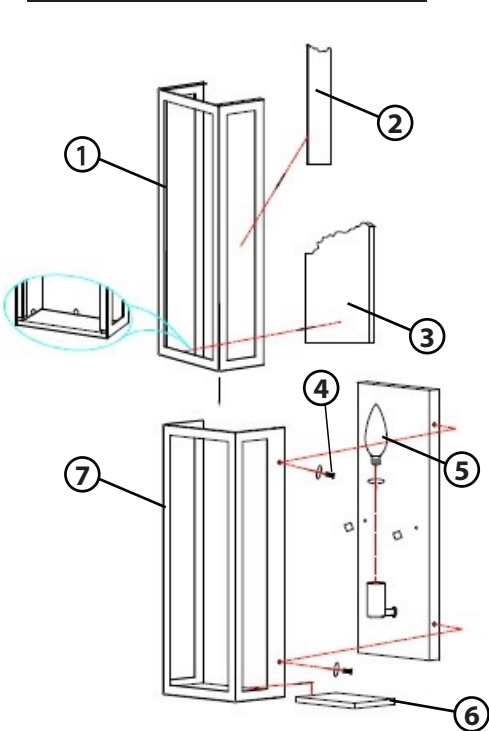
DRAWING 2-Glass install
