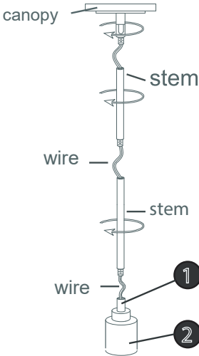
DRAWING 1 - Stem assembly
