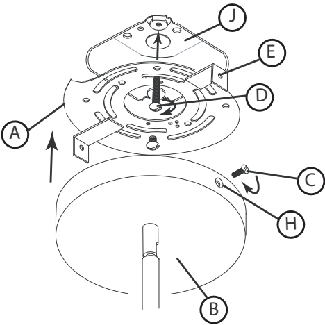
DRAWING 2 - MOUNTING
