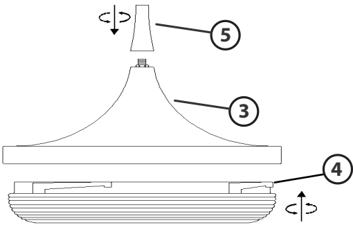
DRAWING 3-GLASS INSTALL
