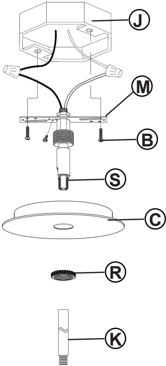
DRAWING 1 - MOUNTING
