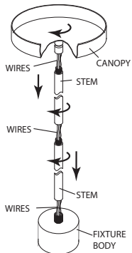
DRAWING 2- Fixture mounting
