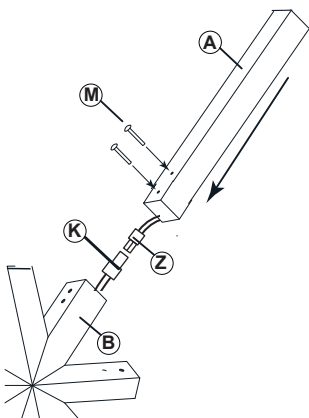
DRAWING 3-LED assembly
