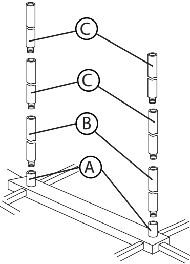
{ DRAWING 2 }
